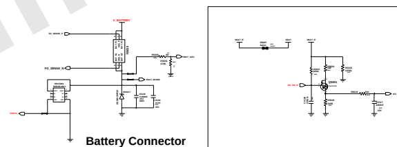
Battery Connector
